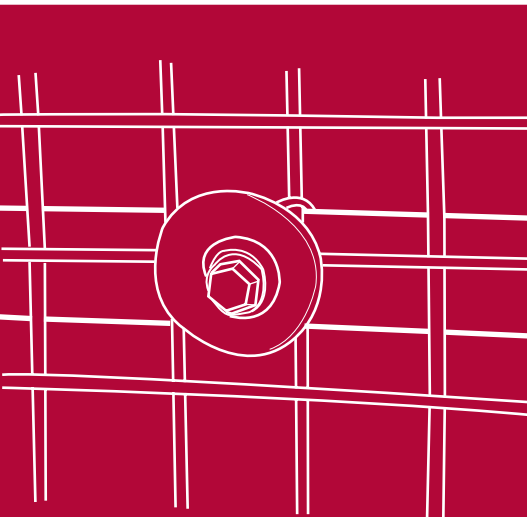
Figure 6: Fixing light mesh
