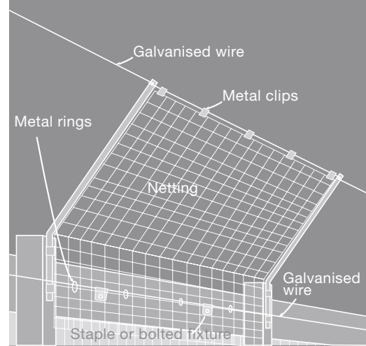
Figure 5: Securing the netting
