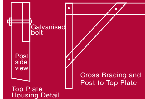
Figure 3: Top plate housing
