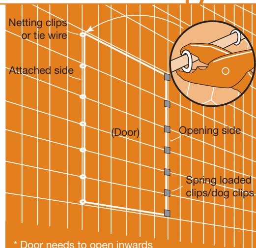
Figure 8: Design and construction of door
