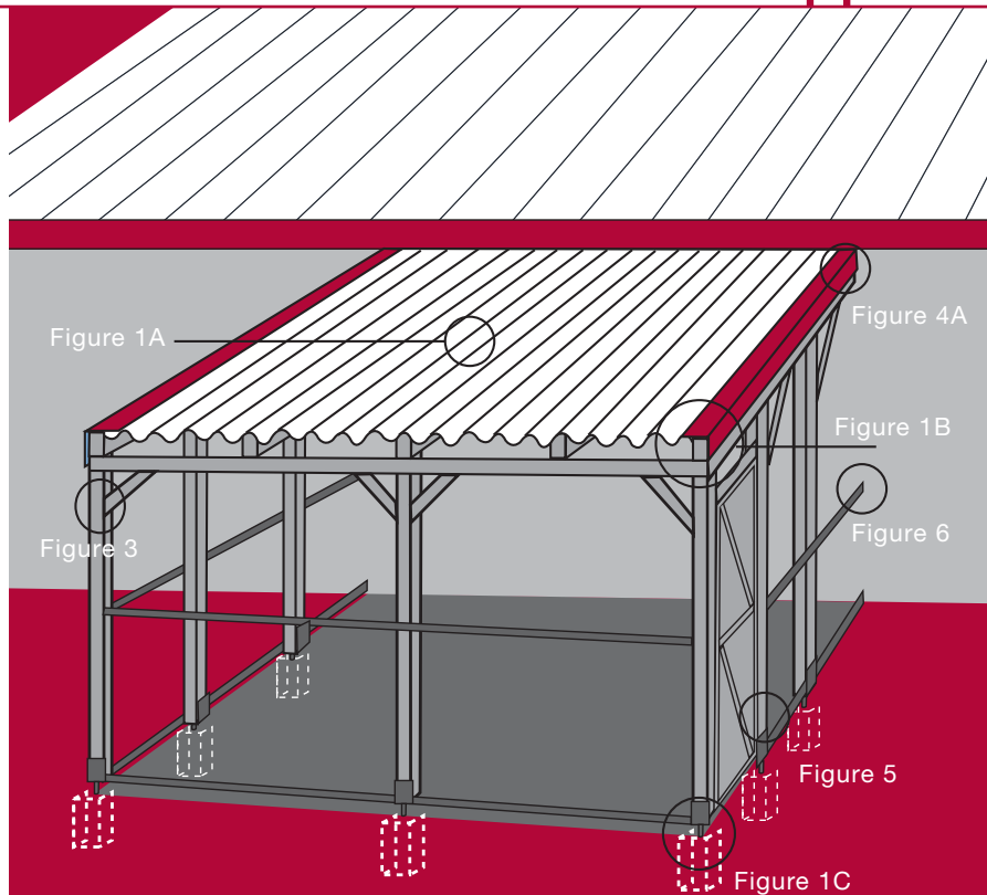
Figure 9: Patio type structure. This shows the basic building structure prior to the addition of solid weatherproof wall cladding on parts of the enclosure (to provide the cat with shelter) and prior to the addition of other features (platforms, climbing planks, scratching posts, beds etc) as described in the text.
