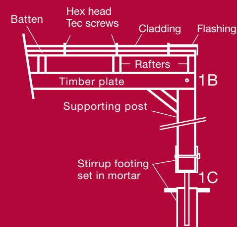
Figure 1: Typical Roof Structure – front view
