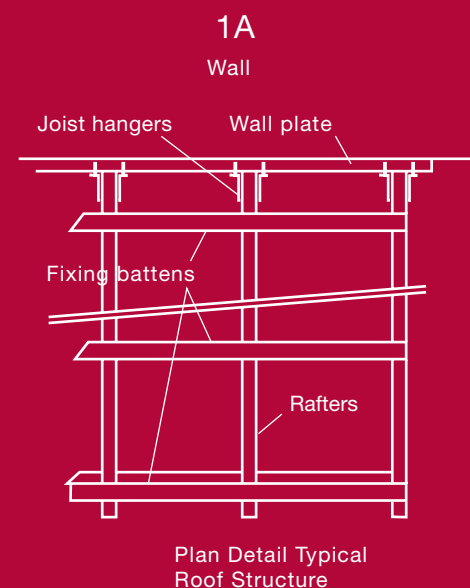
Typical Roof Structure – top view
