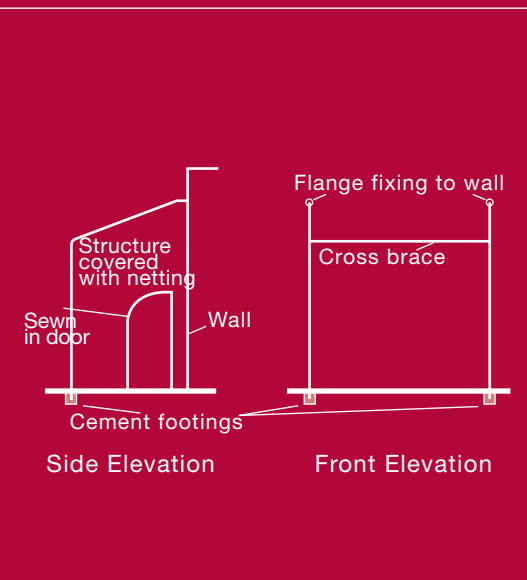
Figure 7: Tubular steel enclosure
